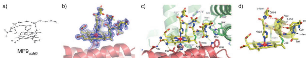
Figure 3. a) Molecular connectivity of MP9 cb562 . b) 2F_o - F_c electron density map corresponding to MP9 cb562 anchored onto His73 inside the Zn 30 :CFMC-1 12 cavity (blue: 1.1 \sigma , purple: 4 \sigma ). c) Interactions of MP9 cb562 with the cavity surface. H-bonding interactions are shown as yellow dashed lines; ordered water molecules are shown as blue spheres. d) Intramolecular H-bonding interactions (red dashed lines) within MP9 cb562 .
